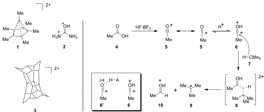
Scheme 2. Dication superelectrophiles
